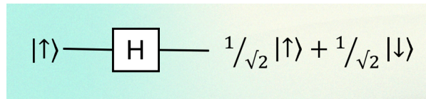
Figure 4: A Hadamard gate takes a pure state as input and converts it into a superposition of eigenstates
