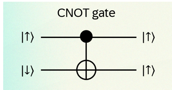
Figure 3: A CNOT gate (conditional NOT) which flips the state of the target qubit only if the state of the control qubit is 1.
