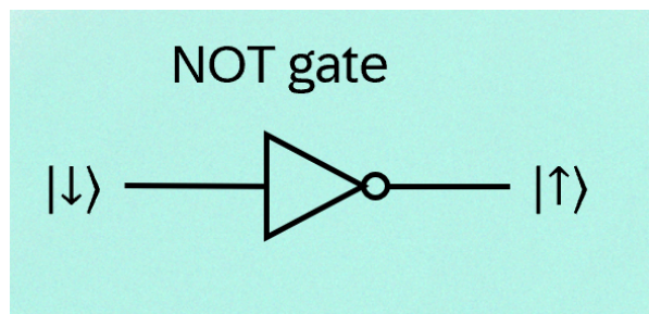
Figure 2: A NOT gate, which turns 0 into 1 and vice versa
