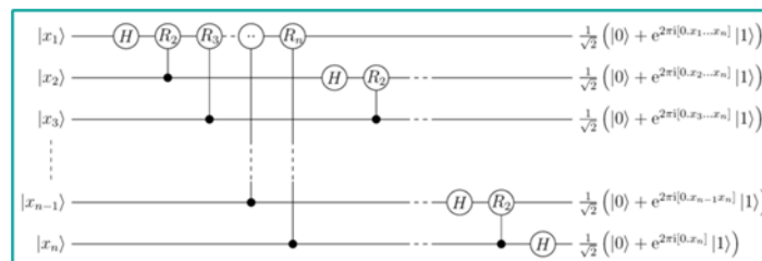
Figure 5: A circuit for a quantum Fourier transform. Source: Wikimedia Commons
