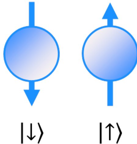
Figure 1: An archetypal qubit: an atom with nuclear spin up or down
