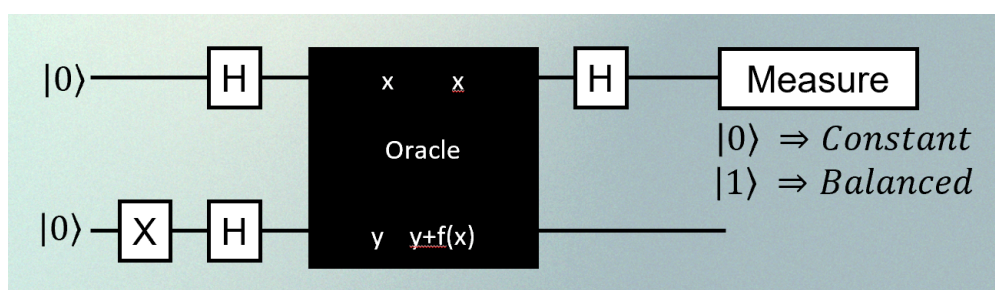
Figure 7: The circuit diagram for an algorithm to solve Deutsch's problem with a single measurement
